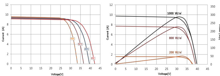
[I-V Curves for 290]
